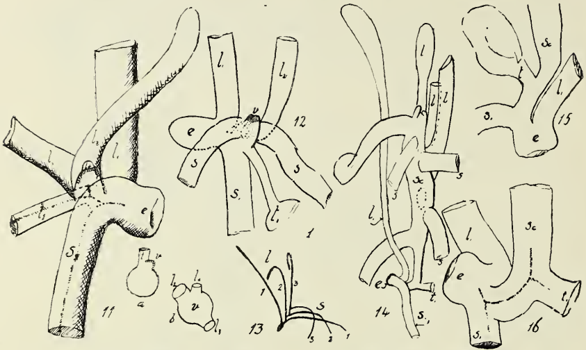
Figs. 11. Polypompholyx. Young protocorm produced at the base of the primary trap, on the base of the primary stolon: t , trap; s , stolon; e , embryo; l , leaf; l 3 must be regarded as transparent: a , diagram, section of primary stolon to show relative positions of first trap and protocorm; b , positions of leaves 2-4 on the protocorm (approx.); v , growing point of protocorm. 12. U. capensis : The same relations as seen in fig. 11. 13. Diagram to show succession of leaves and stolons in a seedling of U. bifida . 14. Somewhat advanced seedling of Polypompholyx; sc , protocorm which at length ends in a scape. 15. The basal portion of a similar seedling of Polypompholyx to show the protocorm united with the stalk of the primary trap, and both arising from the primary stolon. 16. Detail of the seed region of fig. 14.
